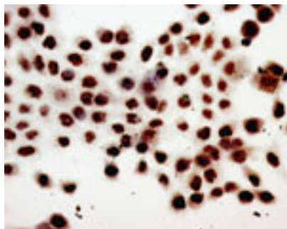
Immunohistochemical detection of PCNA in paraffin embedded HELA cell sections using Mouse monoclonal antibody to PCNA (M-990-100) at 0.4-1.0 µg/ml. Secondary antibody was biotinylated goat anti-mouse at a concentration of 10.0 µg/ml.
