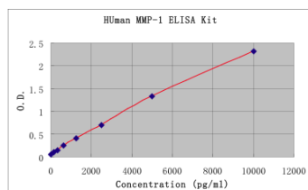
Typical Human MMP-1 ELISA Kit Standard Curve (TMB reaction incubated at 37°C for 12 min)
